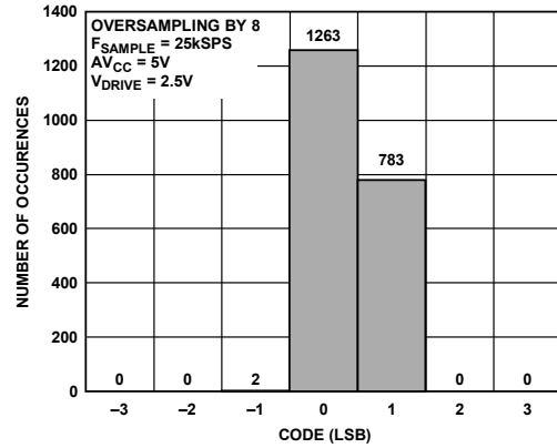
Figure 52. Histogram of Codes—OS x 8 (Three Codes)
