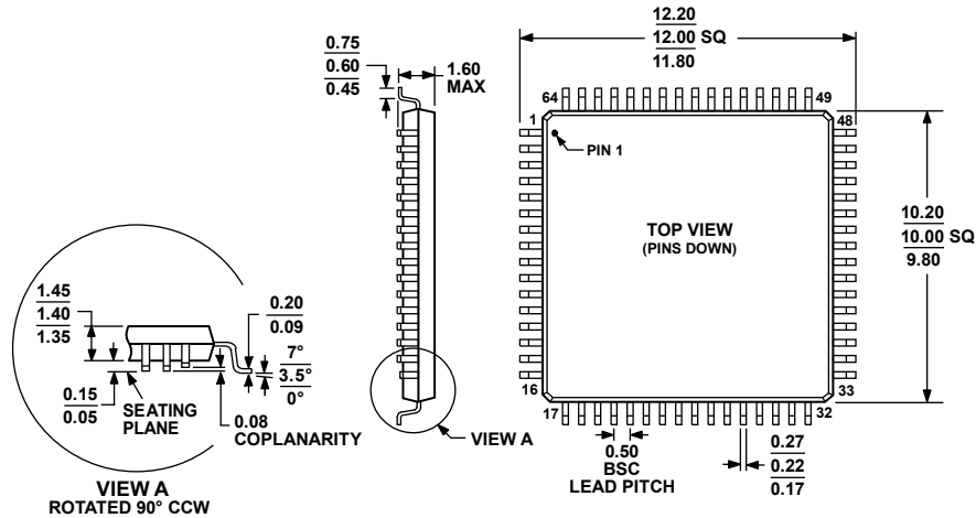
COMPLIANT TO JEDEC STANDARDS MS-026-BCD Figure 65. 64-Lead Low Profile Quad Flat Package [LQFP] (ST-64-2) Dimensions shown in millimetres
